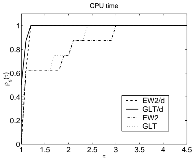
Figure 2: Performance profile of Algorithm 1 and NDNG
