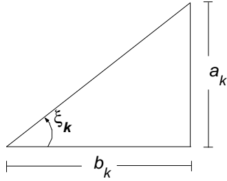
Figure 1: Geometric motivation
